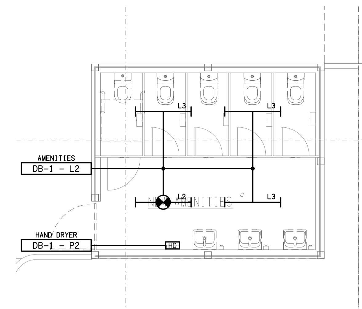
NEW AMENITIES FLOOR / REFLECTED CEILING PLAN SCALE 1:50
