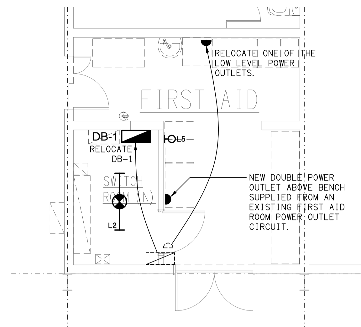
SWITCHROOM FLOOR / REFLECTED CEILING PLAN SCALE 1:50
