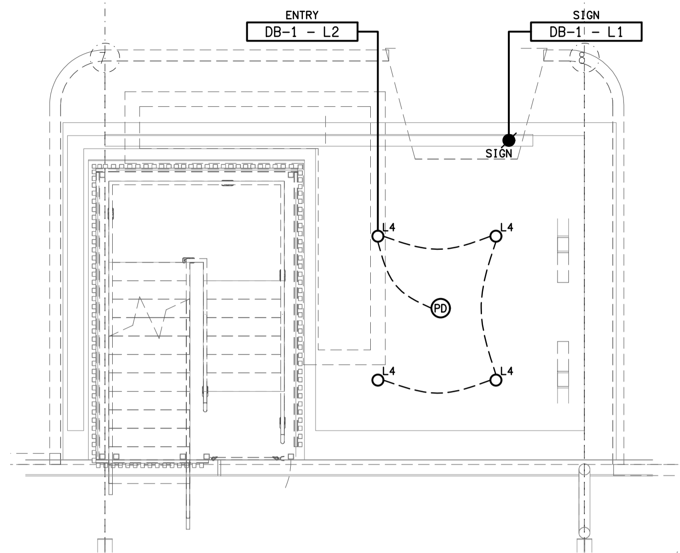
ADMIN ENTRY FLOOR / REFLECTED CEILING PLAN SCALE 1:50
